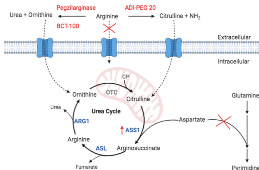
Figure 1. Extracellular metabolism of arginine by BCT-100, pegzilarginase, and ADI-PEG 20 (pegylated bacterial arginine deiminase) reduces cellular uptake of free arginine, resulting in upregulation of argininosuccinate synthetase 1 (ASS1). Ornithine generated by BCT-100 and pegzilarginase cannot be converted into citrulline outside the liver and intestines as ornithine transcarbamylase (OTC) is not expressed (gray); therefore, arginine cannot be synthesized and utilized for viral replication. In contrast, citrulline produced by ADI-PEG 20 is more easily converted to arginine outside the liver since ASS1 and arginosuccinate lyase (ASL) are expressed in most tissues; therefore, viral replication may not be impeded as effectively. A consequence of ASS1 upregulation is that any available citrulline will be rapidly conjugated to aspartate, preventing its utilization in pyrimidine ring synthesis, thereby restricting viral replication of another key building block. ARG1, arginase 1; CP, carbamoyl phosphate.
